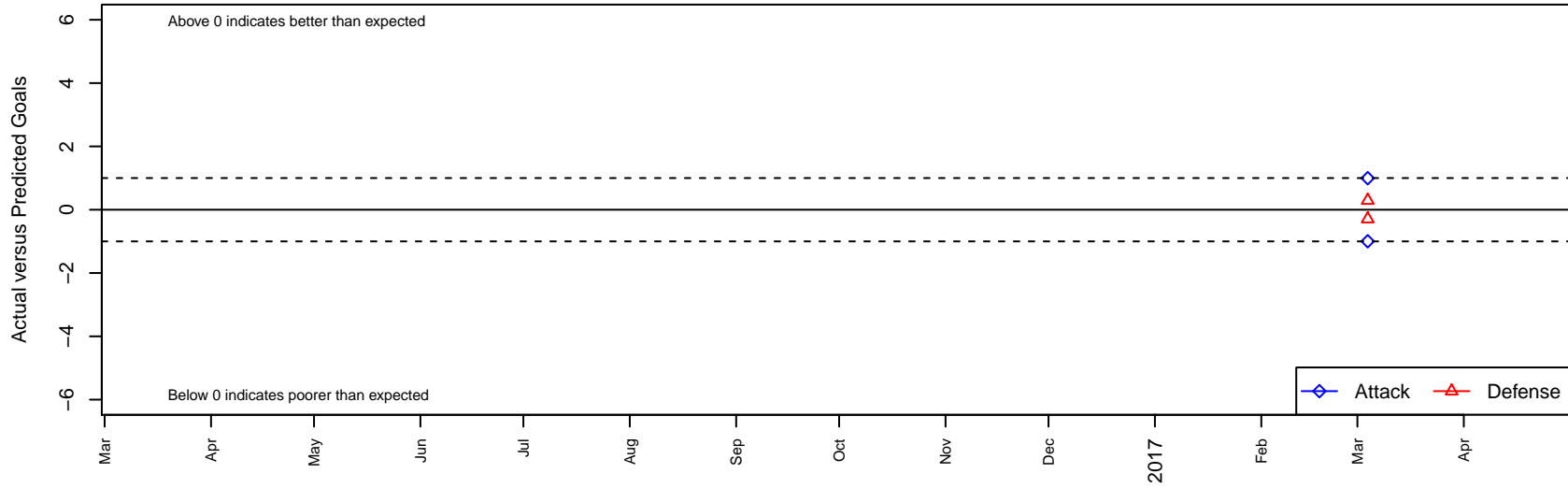
Twin Falls Rapids G04 Dots are actual minus expected GF (blue circles) and GA (red triangles). Blue line is smoothed change in attack strength. Red is smoothed change in defense strength.
